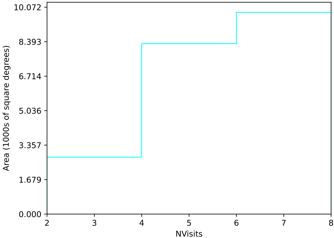
too_elab_r8_d3_giz_v3.4_10yrs Yr 1 u band: NVisits
