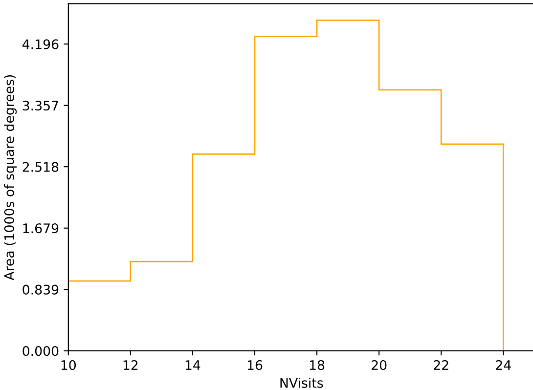
too_elab_r8_d3_giz_v3.4_10yrs Yr 1 r band: NVisits
