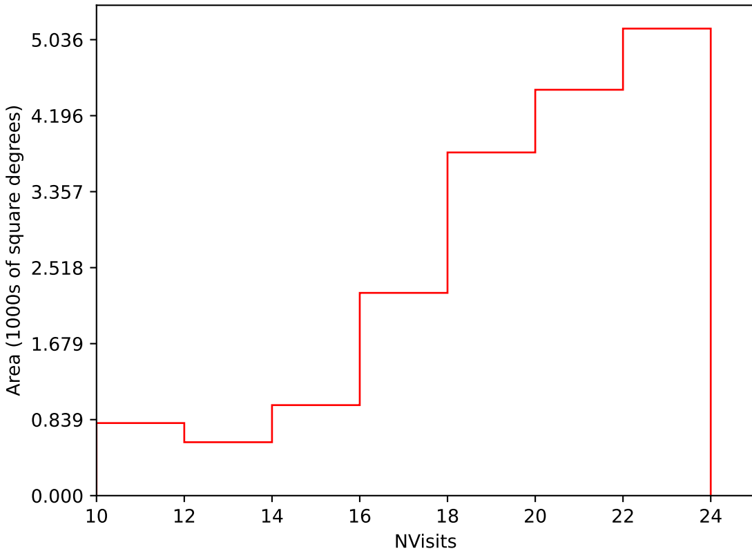
too_elab_r8_d3_giz_v3.4_10yrs Yr 1 i band: NVisits
