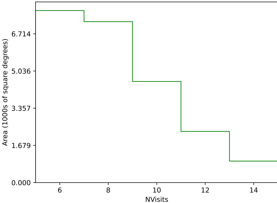
too_elab_r8_d3_giz_v3.4_10yrs Yr 1 g band: NVisits
