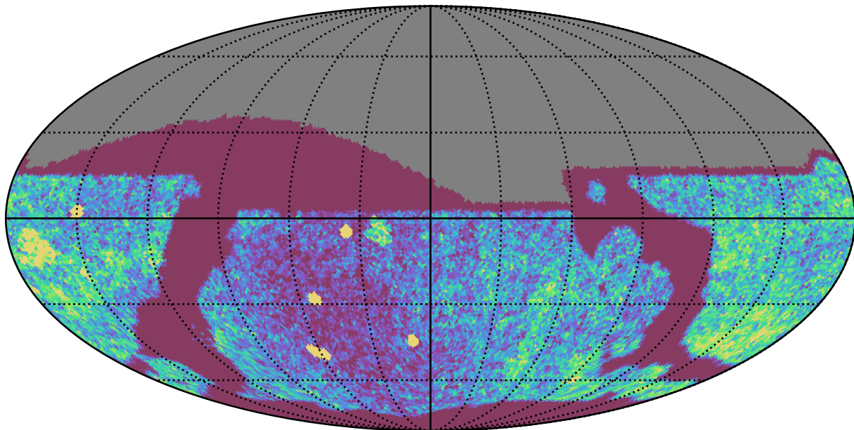
too_elab_r8_d3_giz_v3.4_10yrs Yr 1 all bands: NVisits
