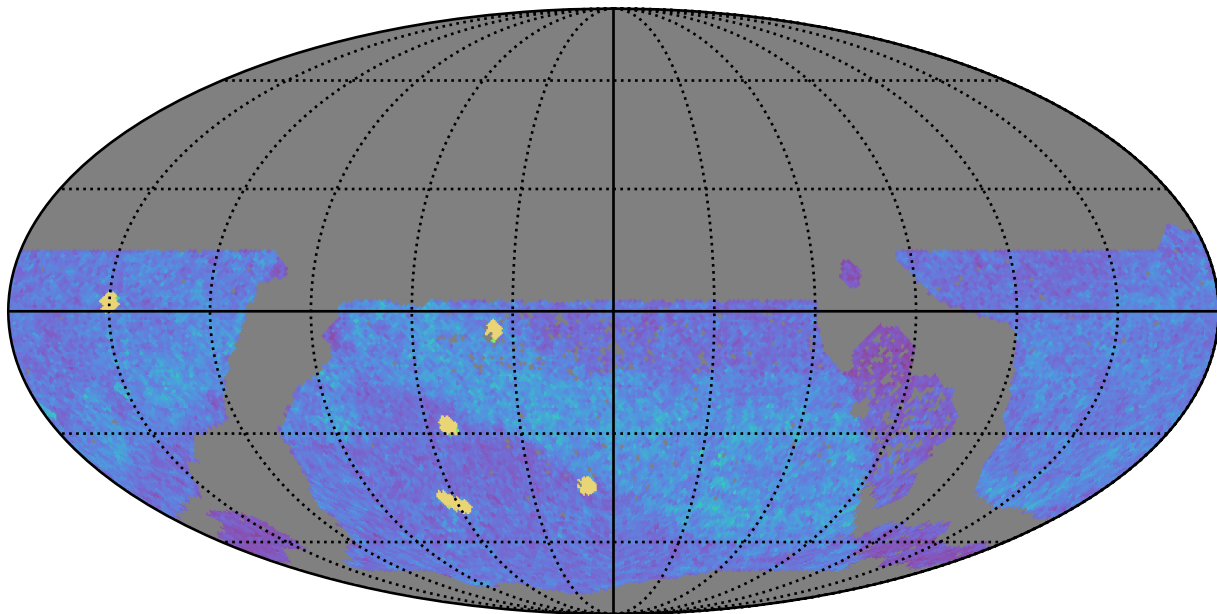
too_elab_r8_d3_giz_v3.4_10yrs WFD z band: NVisits
