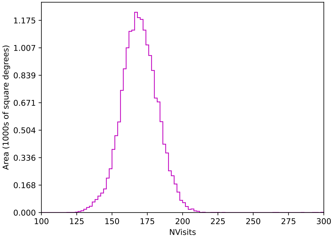
too_elab_r8_d3_giz_v3.4_10yrs WFD z band: NVisits
