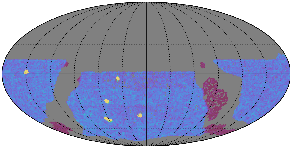
too_elab_r8_d3_giz_v3.4_10yrs WFD y band: NVisits
