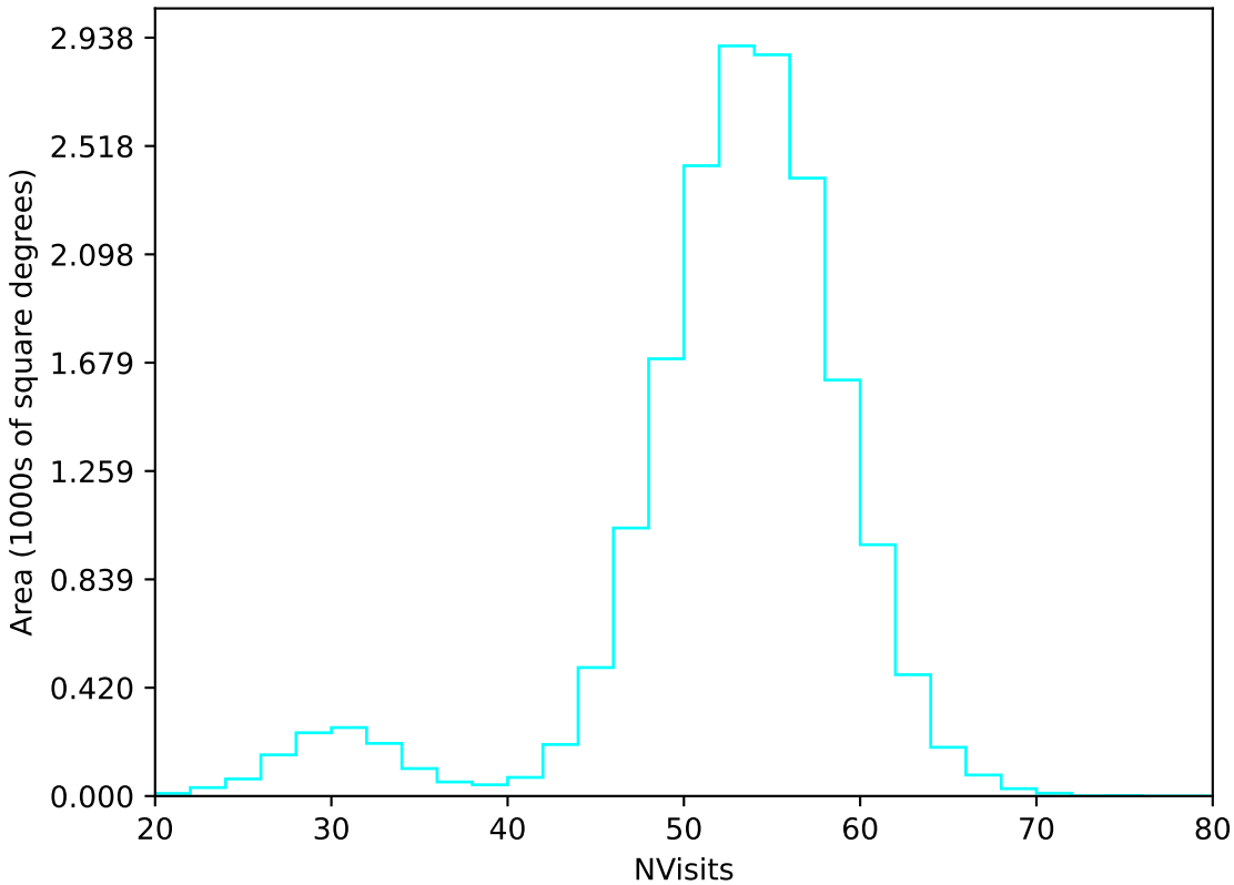
too_elab_r8_d3_giz_v3.4_10yrs WFD u band: NVisits
