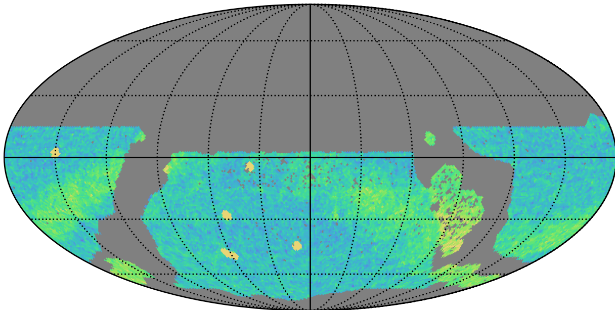
too_elab_r8_d3_giz_v3.4_10yrs WFD r band: NVisits
