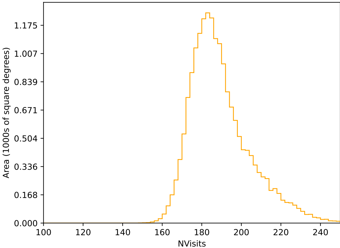
too_elab_r8_d3_giz_v3.4_10yrs WFD r band: NVisits
