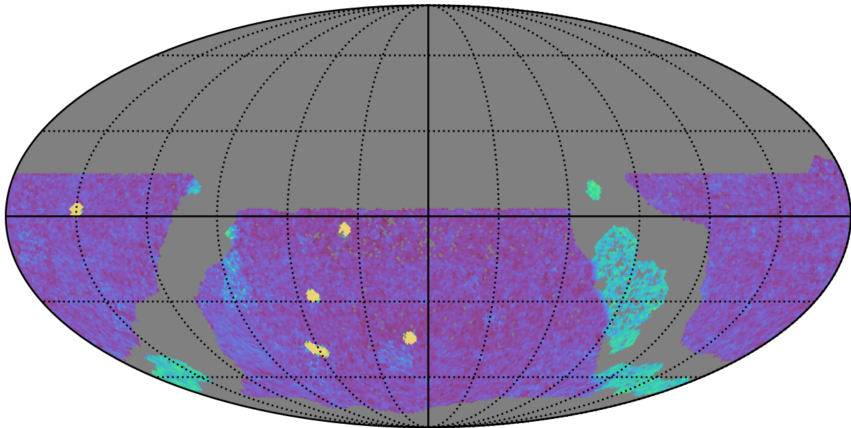
too_elab_r8_d3_giz_v3.4_10yrs WFD g band: NVisits
