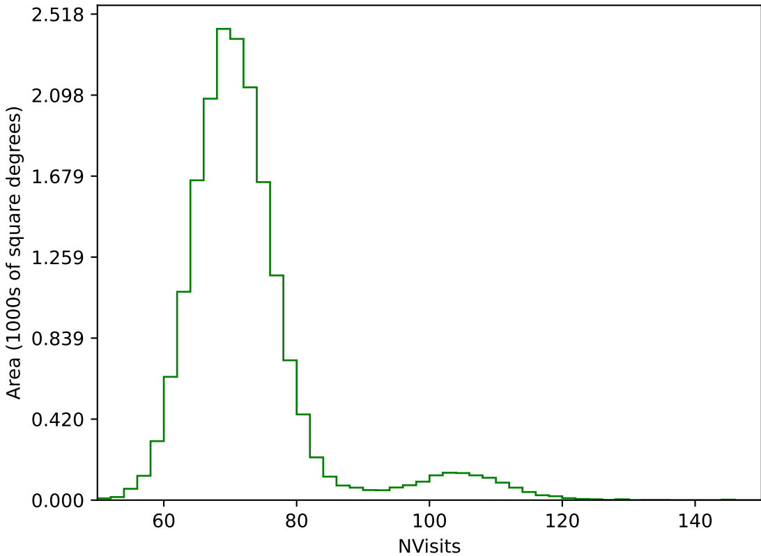
too_elab_r8_d3_giz_v3.4_10yrs WFD g band: NVisits
