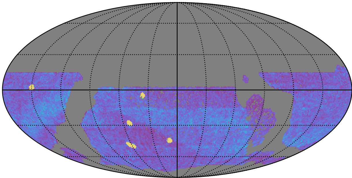
too_elab_r8_d3_giz_v3.4_10yrs WFD all bands: NVisits
