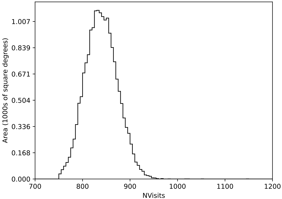
too_elab_r8_d3_giz_v3.4_10yrs WFD all bands: NVisits
