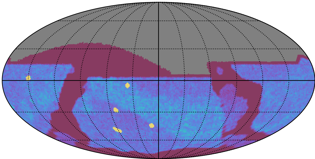
too_elab_r8_d3_giz_v3.4_10yrs All sky z band: NVisits
