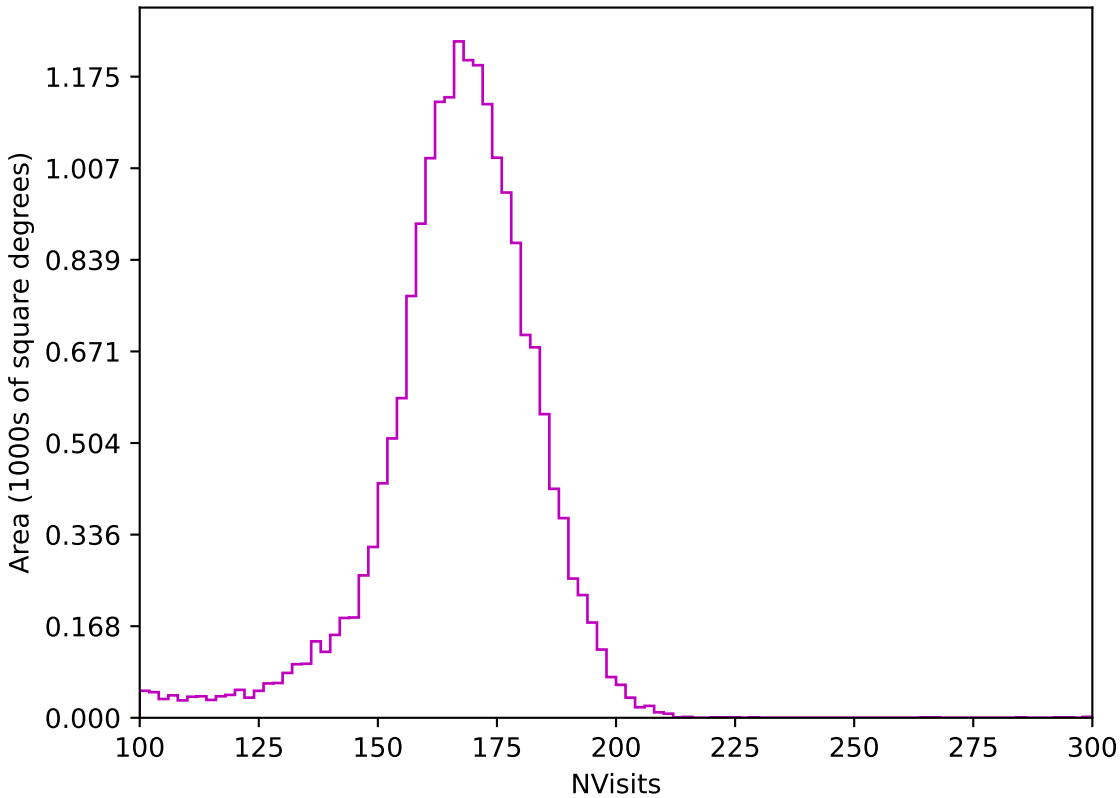
too_elab_r8_d3_giz_v3.4_10yrs All sky z band: NVisits
