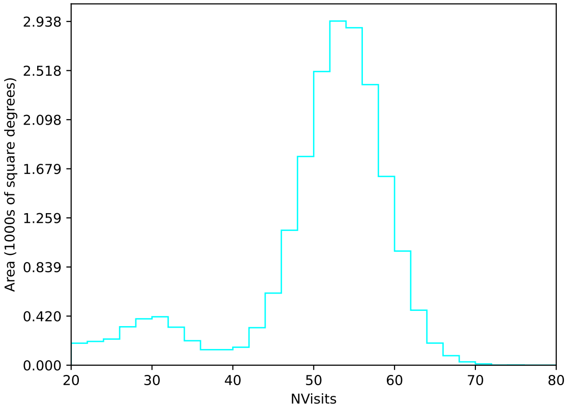
too_elab_r8_d3_giz_v3.4_10yrs All sky u band: NVisits
