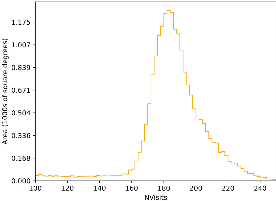
too_elab_r8_d3_giz_v3.4_10yrs All sky r band: NVisits
