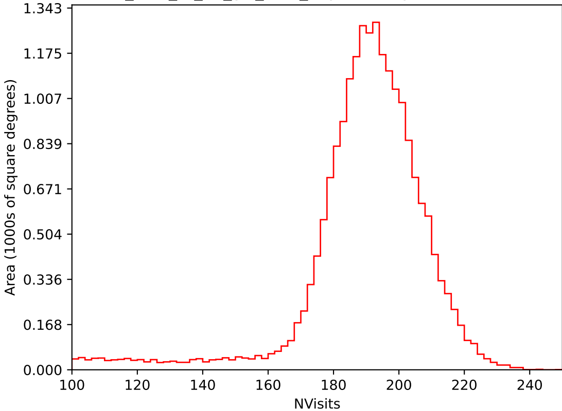
too_elab_r8_d3_giz_v3.4_10yrs All sky i band: NVisits
