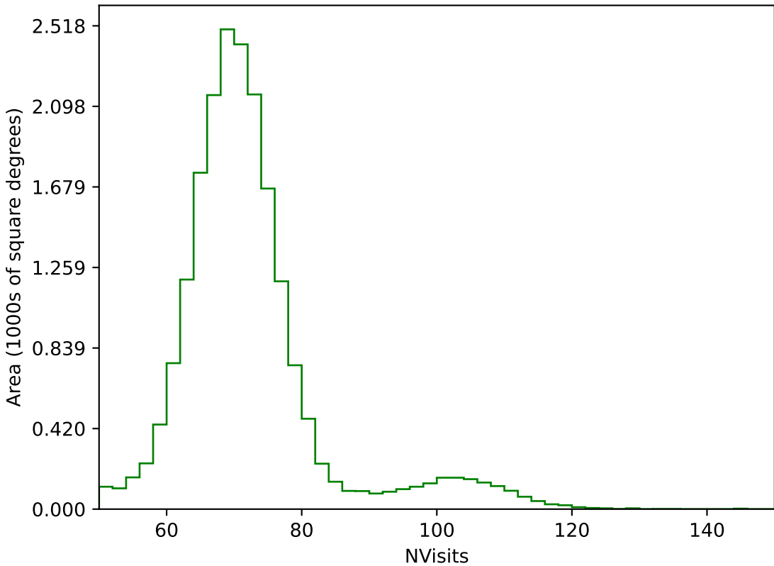
too_elab_r8_d3_giz_v3.4_10yrs All sky g band: NVisits
