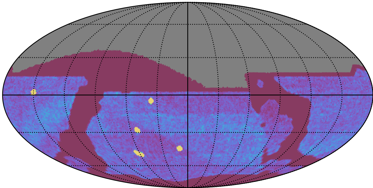
too_elab_r8_d3_giz_v3.4_10yrs All sky all bands: NVisits
