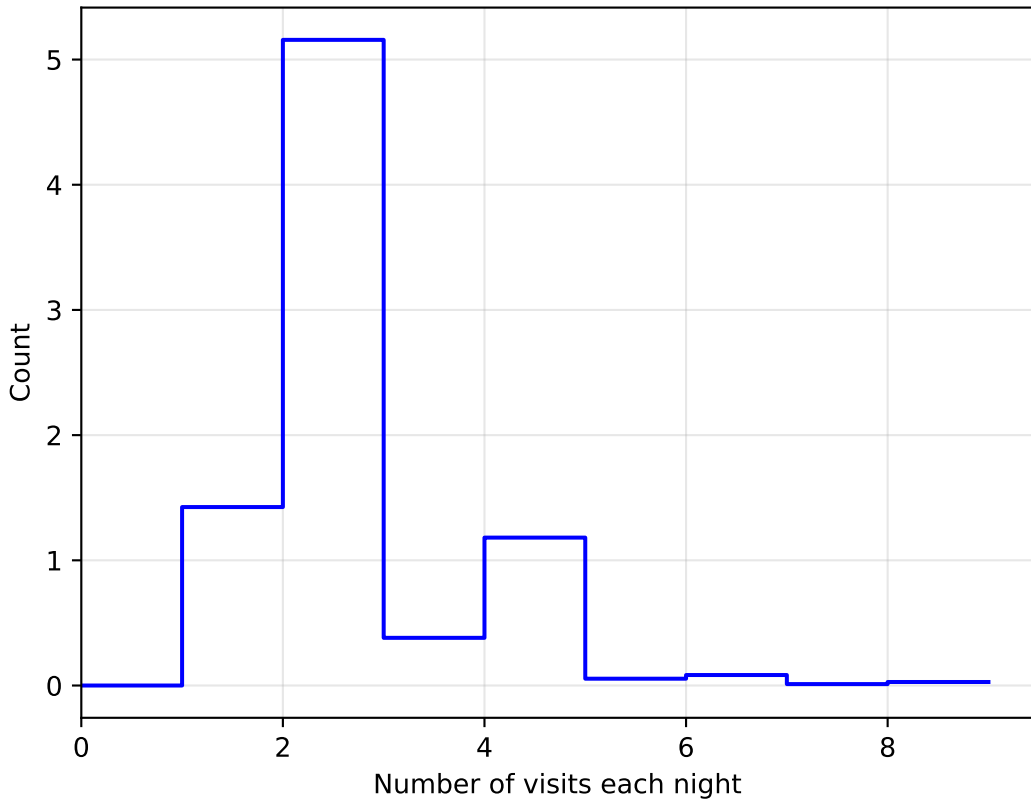
1e6 too_elab_r8_d3_giz_v3.4_10yrs WFD: NVisitsPerNight
