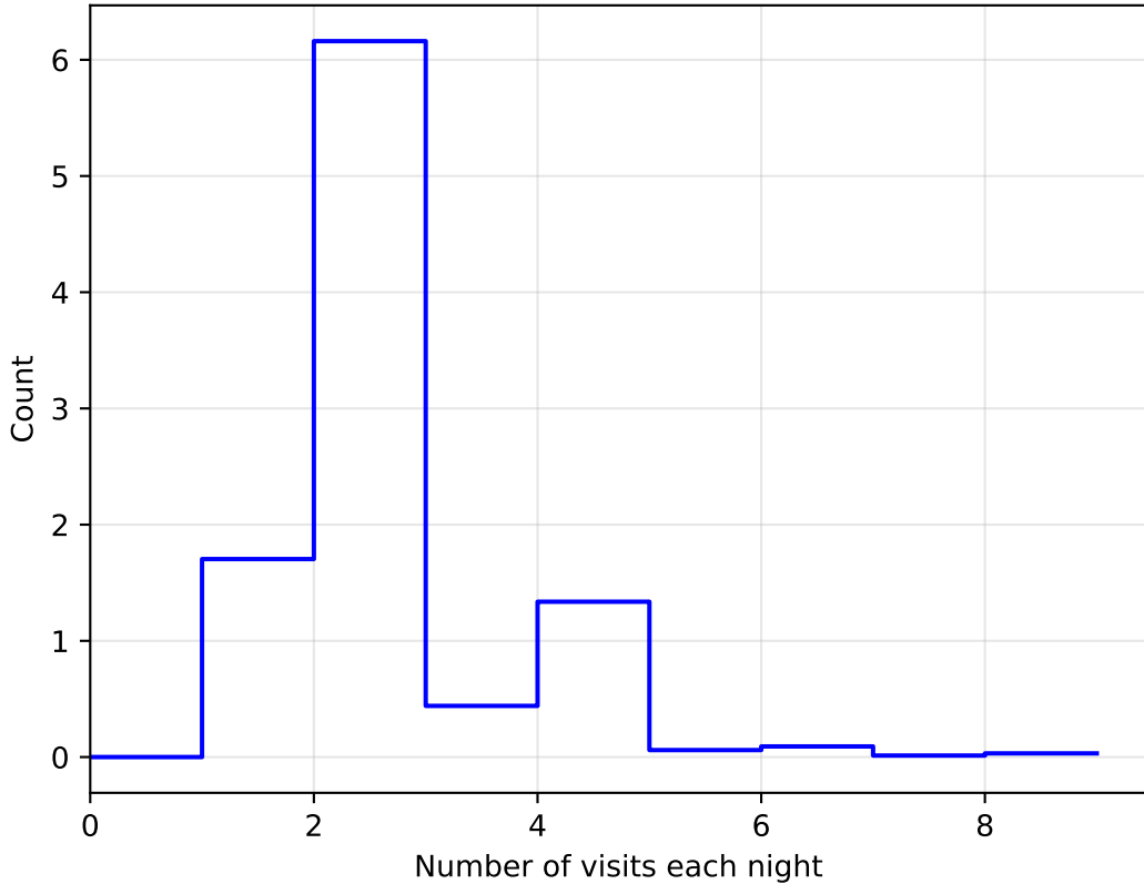
too_elab_r8_d3_giz_v3.4_10yrs All sky: NVisitsPerNight
