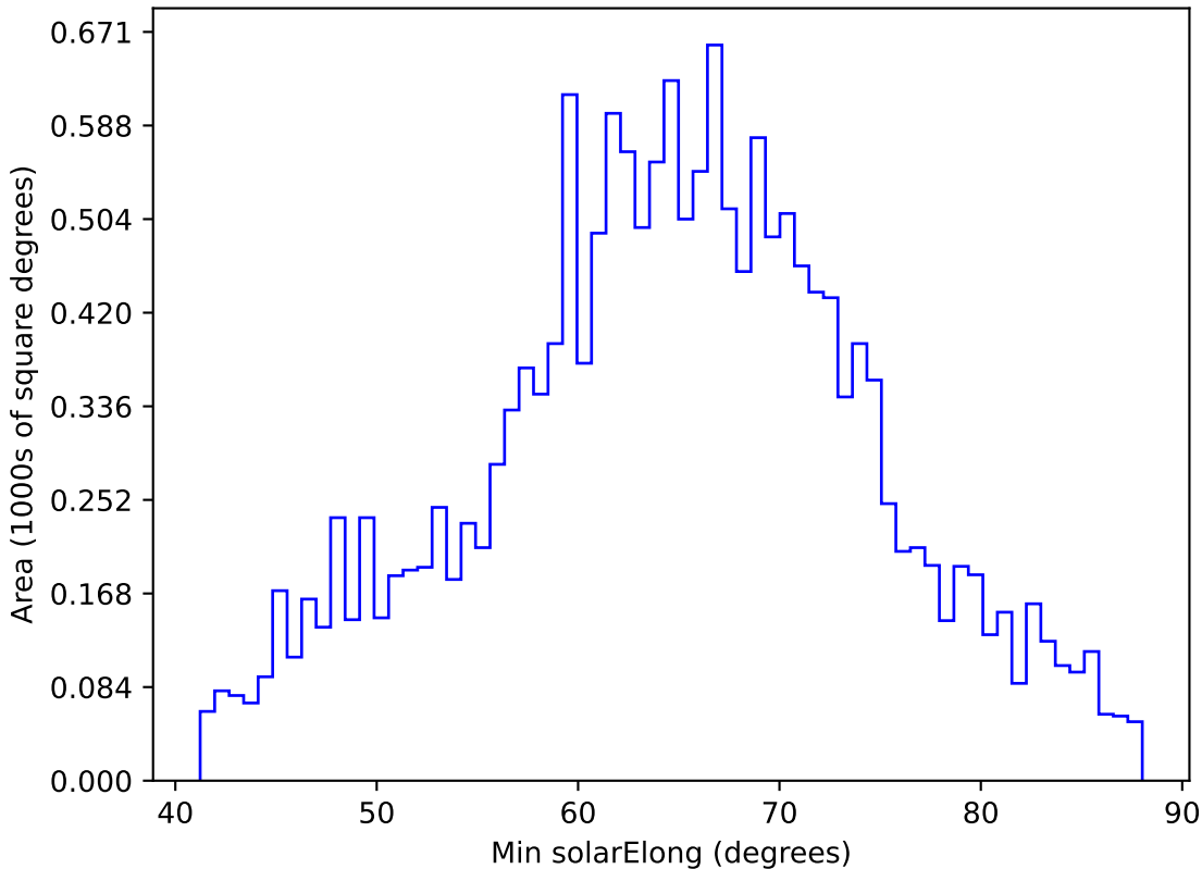
too_elab_r8_d3_giz_v3.4_10yrs WFD y band: Min solarElong
