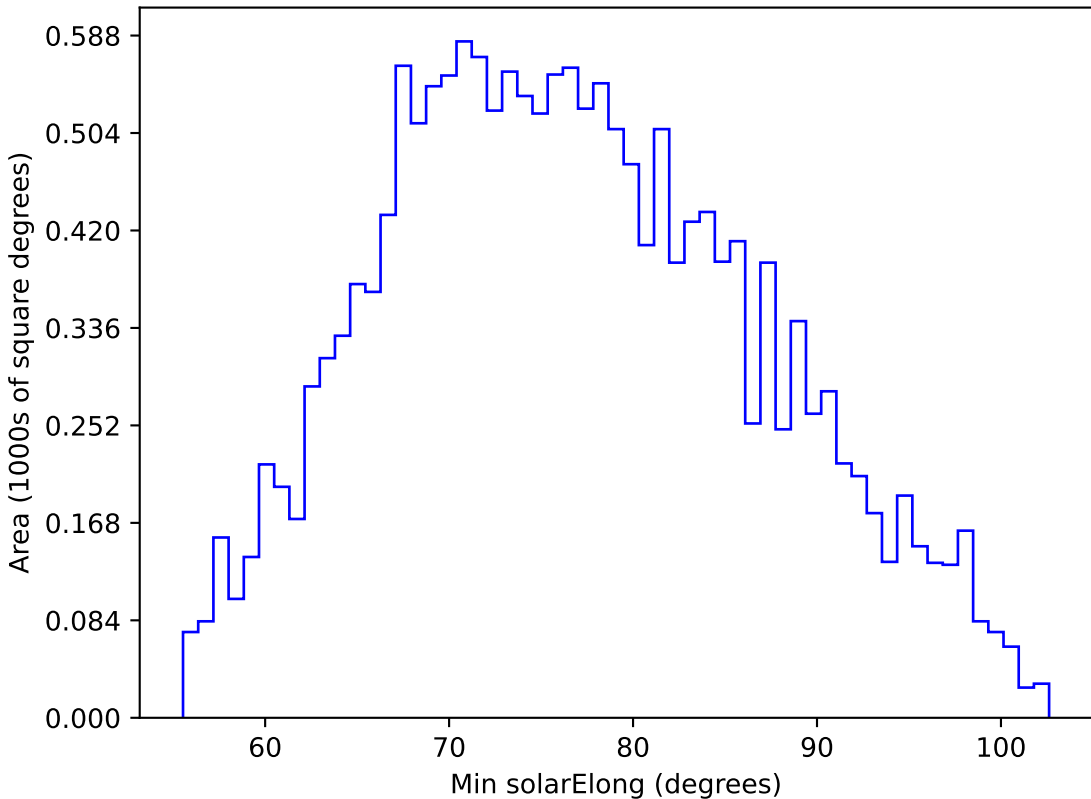
too_elab_r8_d3_giz_v3.4_10yrs WFD u band: Min solarElong
