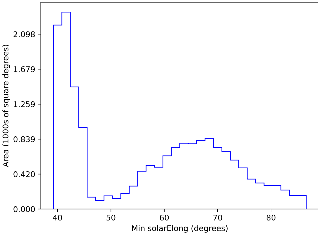
too_elab_r8_d3_giz_v3.4_10yrs WFD r band: Min solarElong
