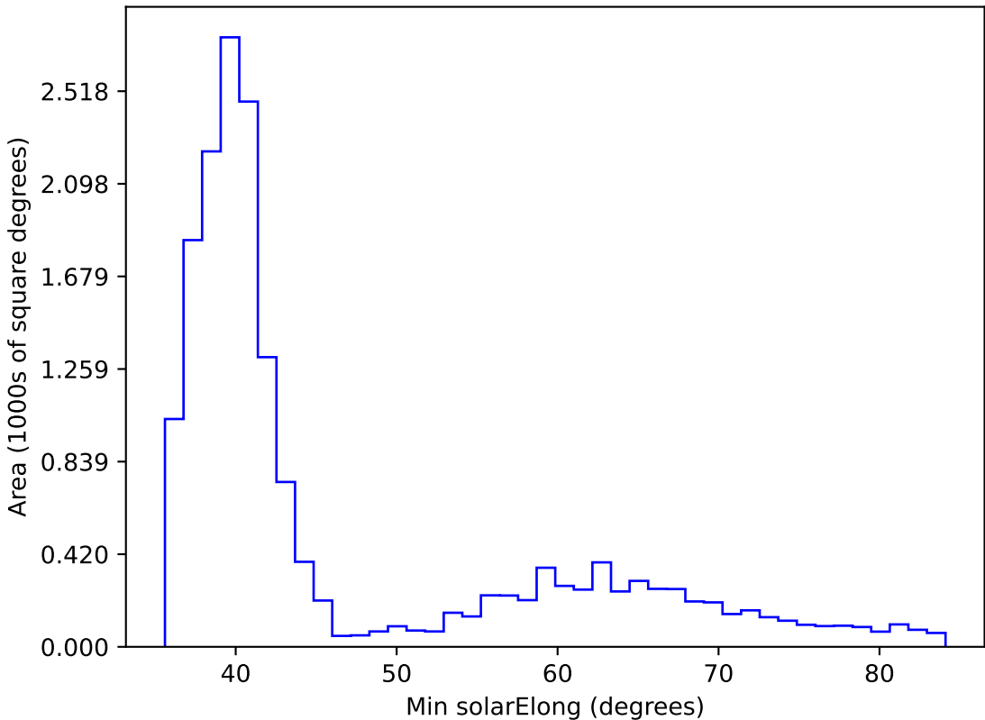
too_elab_r8_d3_giz_v3.4_10yrs WFD all bands: Min solarElong
