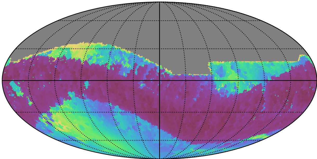
too_elab_r8_d3_giz_v3.4_10yrs All sky z band: Min solarElong
