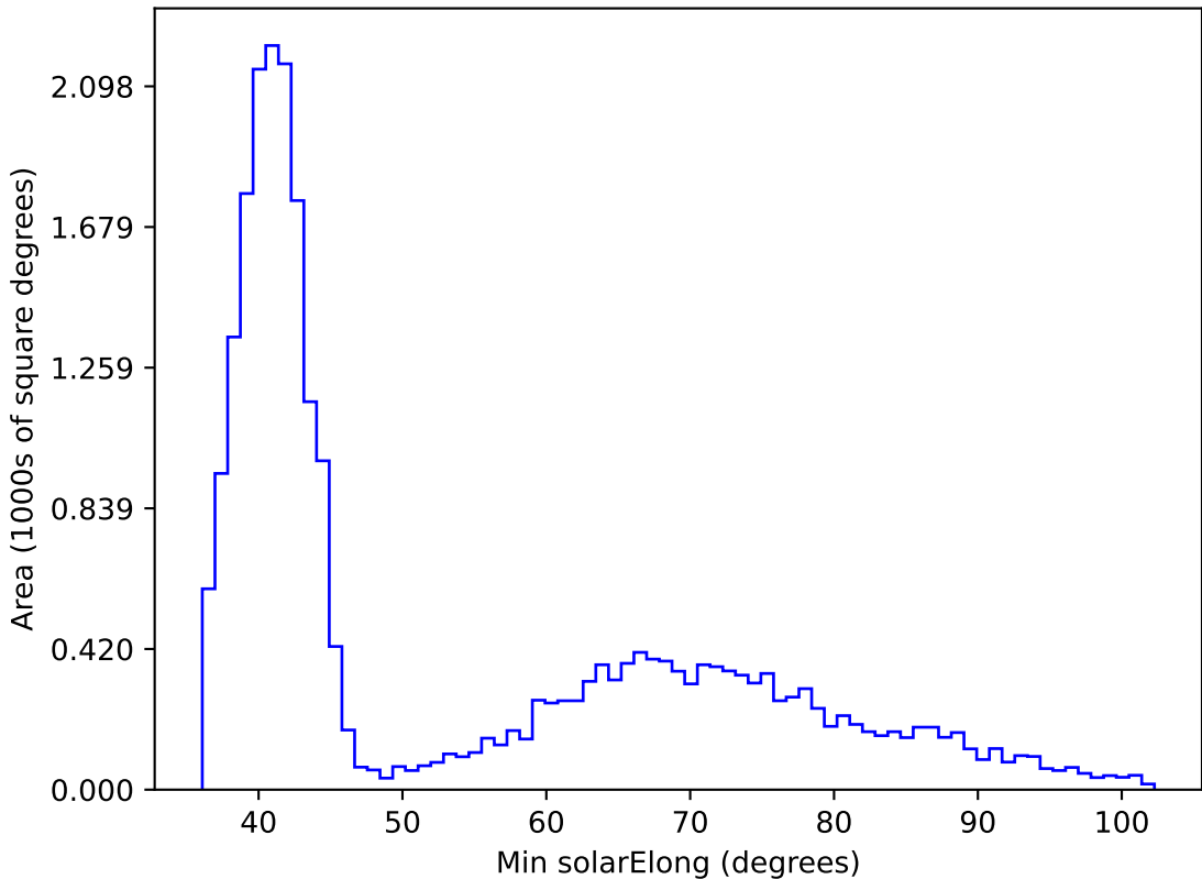
too_elab_r8_d3_giz_v3.4_10yrs All sky z band: Min solarElong
