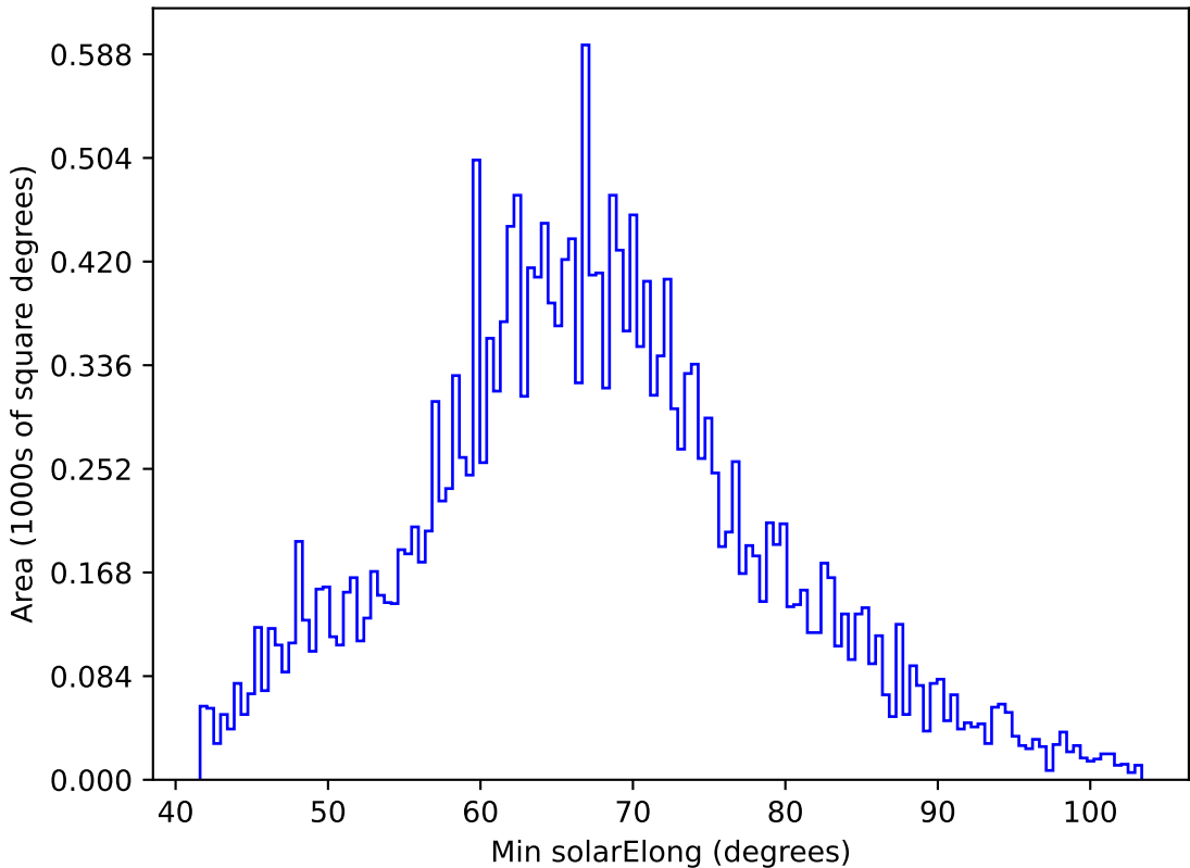
too_elab_r8_d3_giz_v3.4_10yrs All sky y band: Min solarElong
