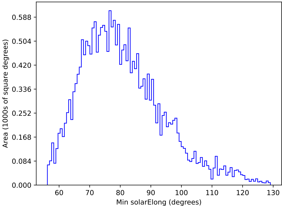
too_elab_r8_d3_giz_v3.4_10yrs All sky u band: Min solarElong
