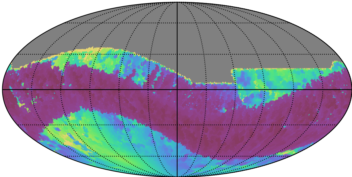
too_elab_r8_d3_giz_v3.4_10yrs All sky i band: Min solarElong
