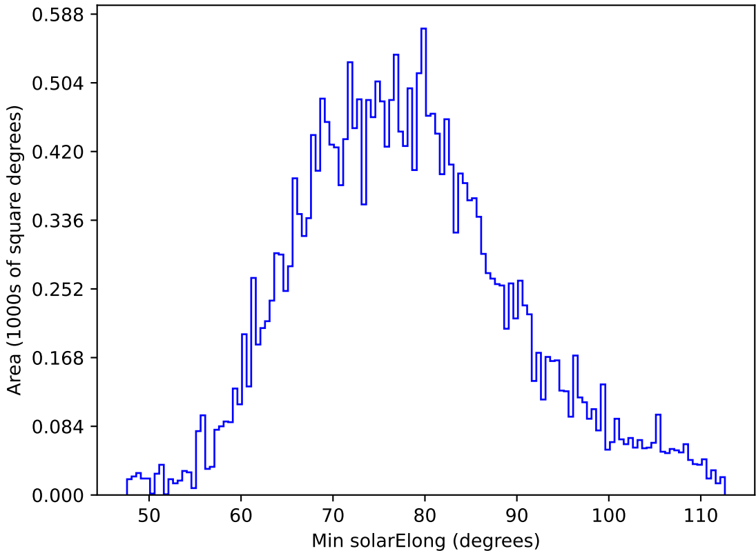
too_elab_r8_d3_giz_v3.4_10yrs All sky g band: Min solarElong
