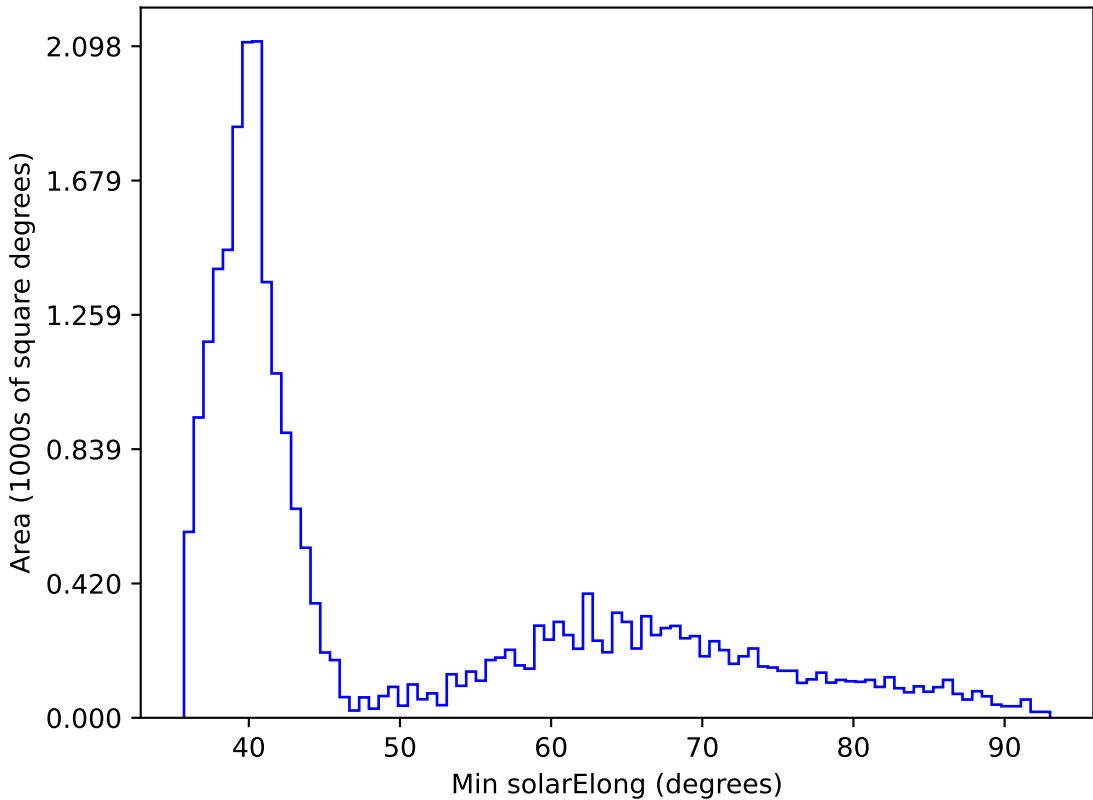
too_elab_r8_d3_giz_v3.4_10yrs All sky all bands: Min solarElong
