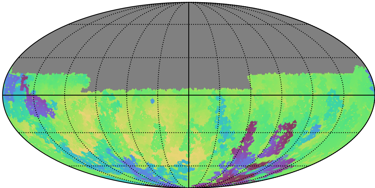
too_elab_r8_d3_giz_v3.4_10yrs Yr 1 u band: Min skyBrightness
