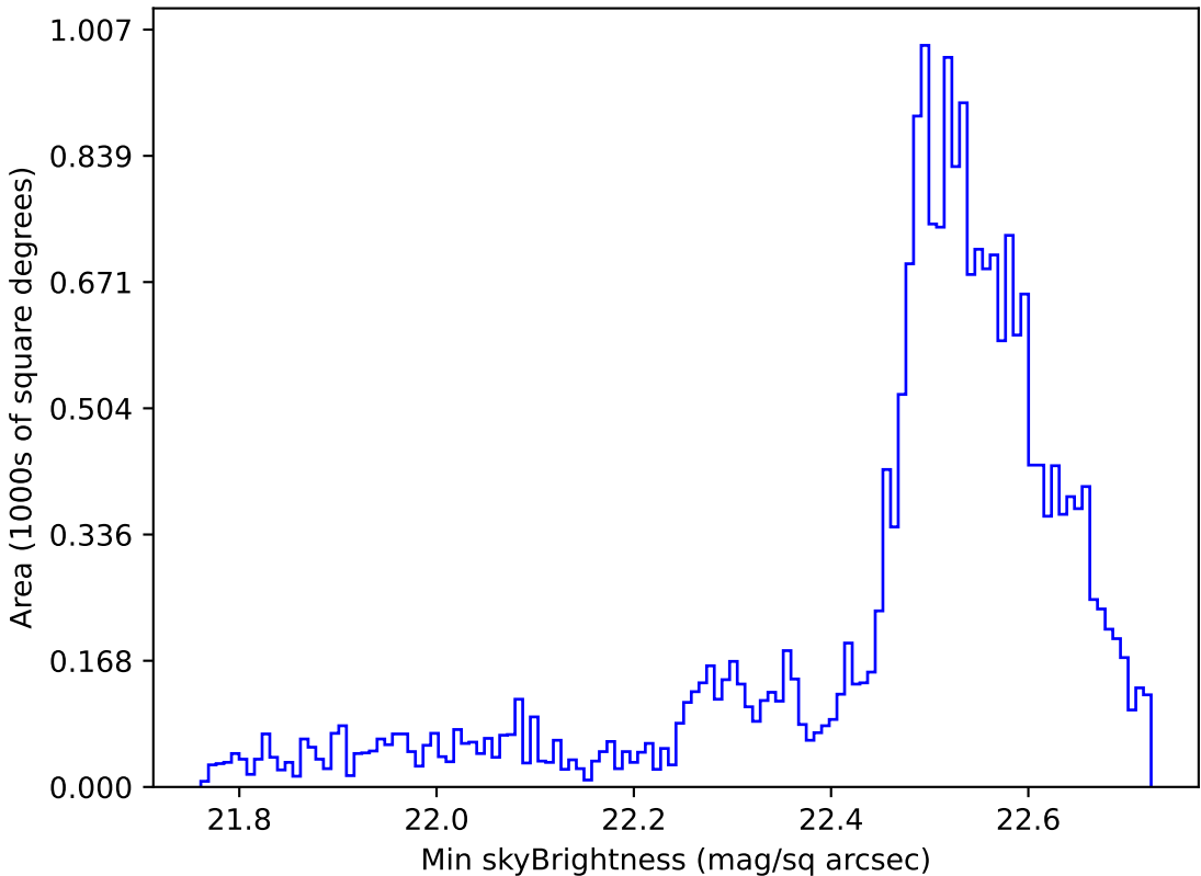
too_elab_r8_d3_giz_v3.4_10yrs Yr 1 u band: Min skyBrightness
