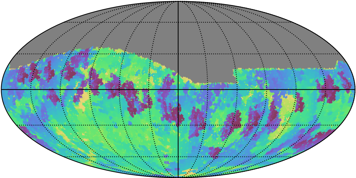
too_elab_r8_d3_giz_v3.4_10yrs Yr 1 i band: Min skyBrightness
