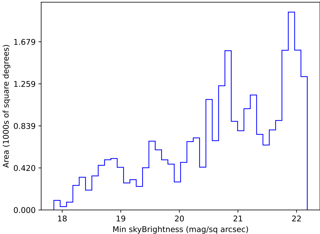
too_elab_r8_d3_giz_v3.4_10yrs Yr 1 g band: Min skyBrightness
