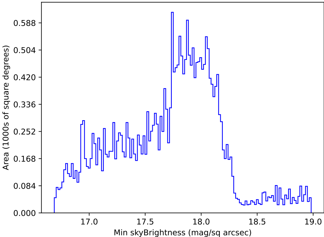
too_elab_r8_d3_giz_v3.4_10yrs Yr 1 all bands: Min skyBrightness
