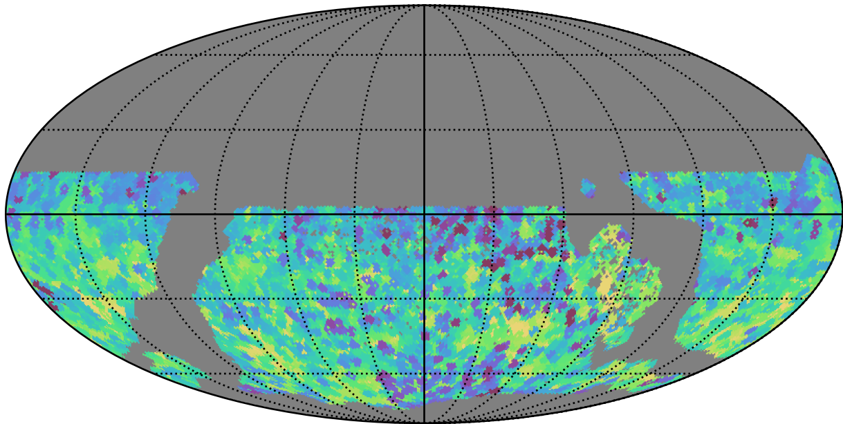
too_elab_r8_d3_giz_v3.4_10yrs WFD y band: Min skyBrightness
