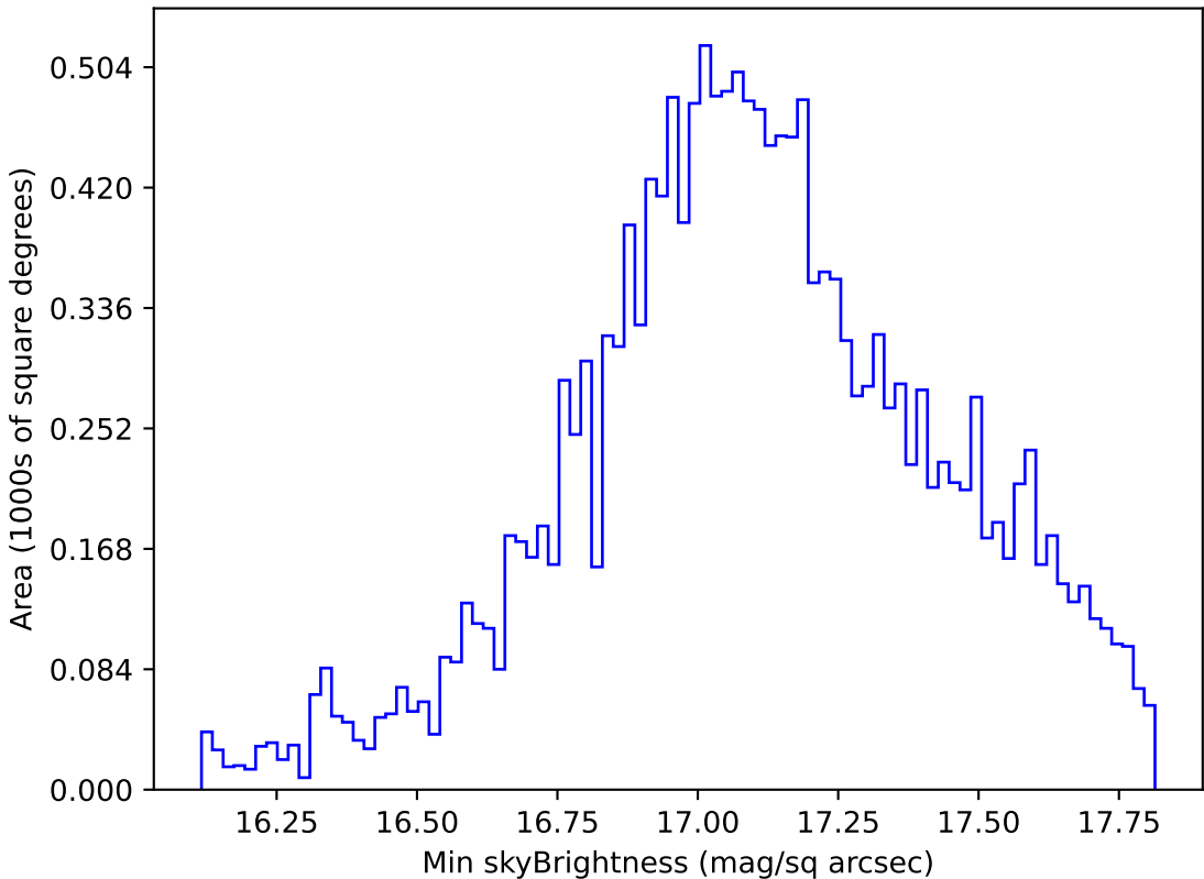
too_elab_r8_d3_giz_v3.4_10yrs WFD y band: Min skyBrightness
