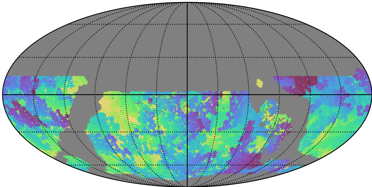
too_elab_r8_d3_giz_v3.4_10yrs WFD u band: Min skyBrightness
