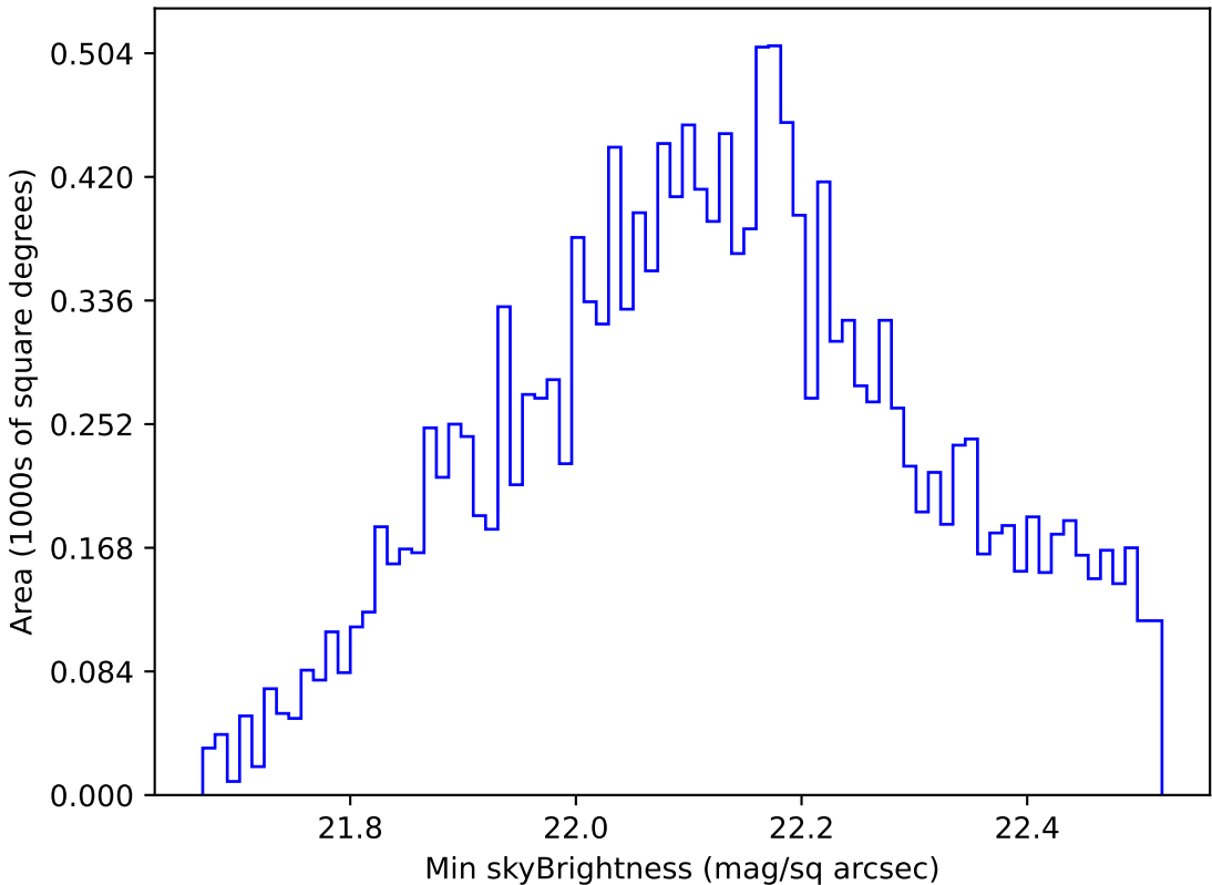
too_elab_r8_d3_giz_v3.4_10yrs WFD u band: Min skyBrightness
