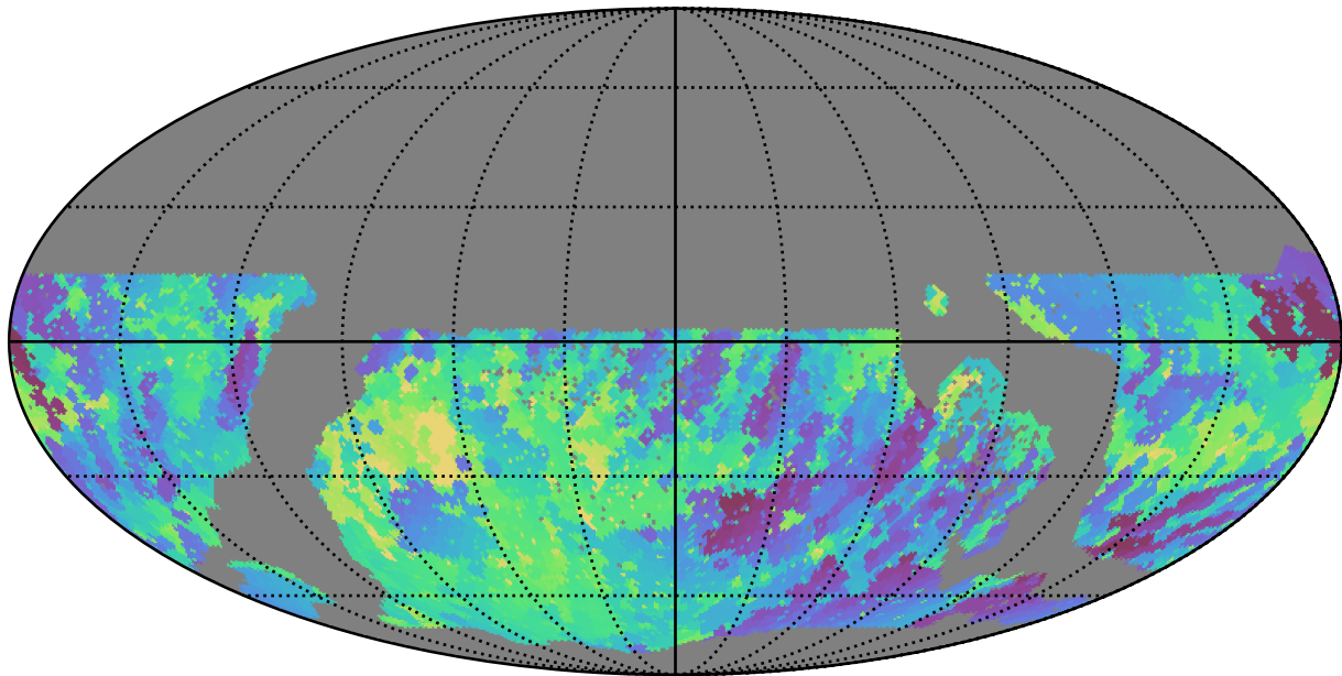
too_elab_r8_d3_giz_v3.4_10yrs WFD r band: Min skyBrightness
