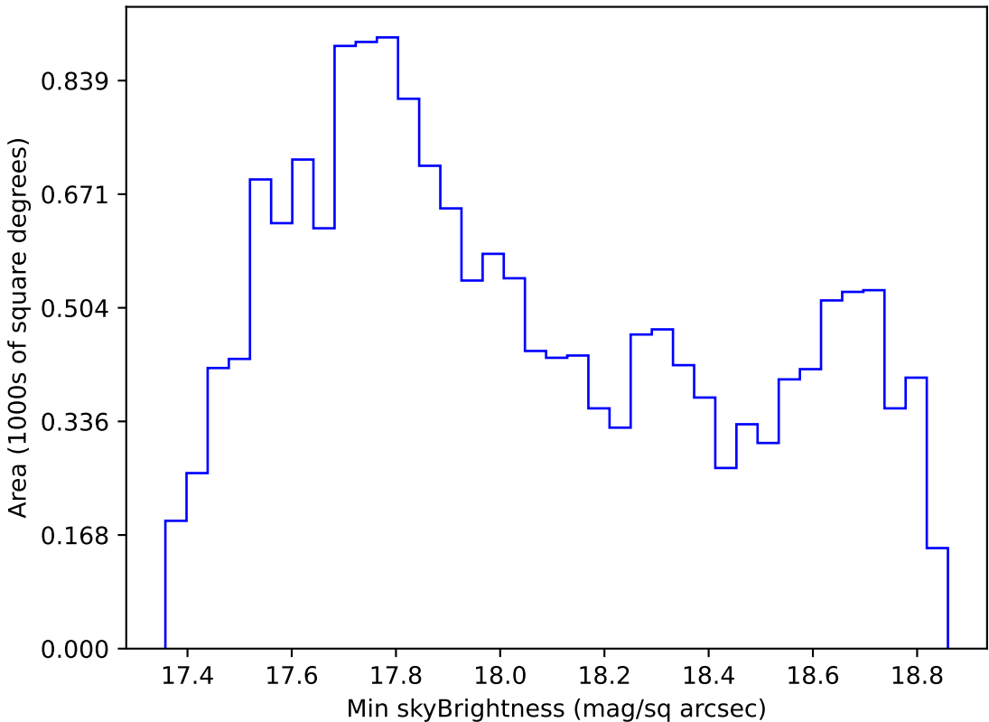
too_elab_r8_d3_giz_v3.4_10yrs WFD i band: Min skyBrightness
