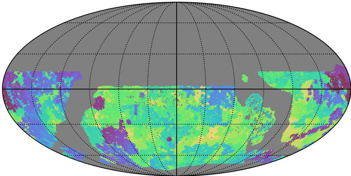
too_elab_r8_d3_giz_v3.4_10yrs WFD g band: Min skyBrightness
