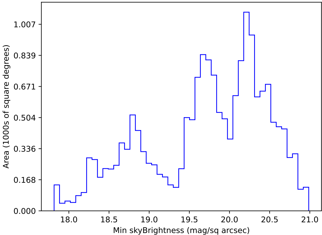
too_elab_r8_d3_giz_v3.4_10yrs WFD g band: Min skyBrightness
