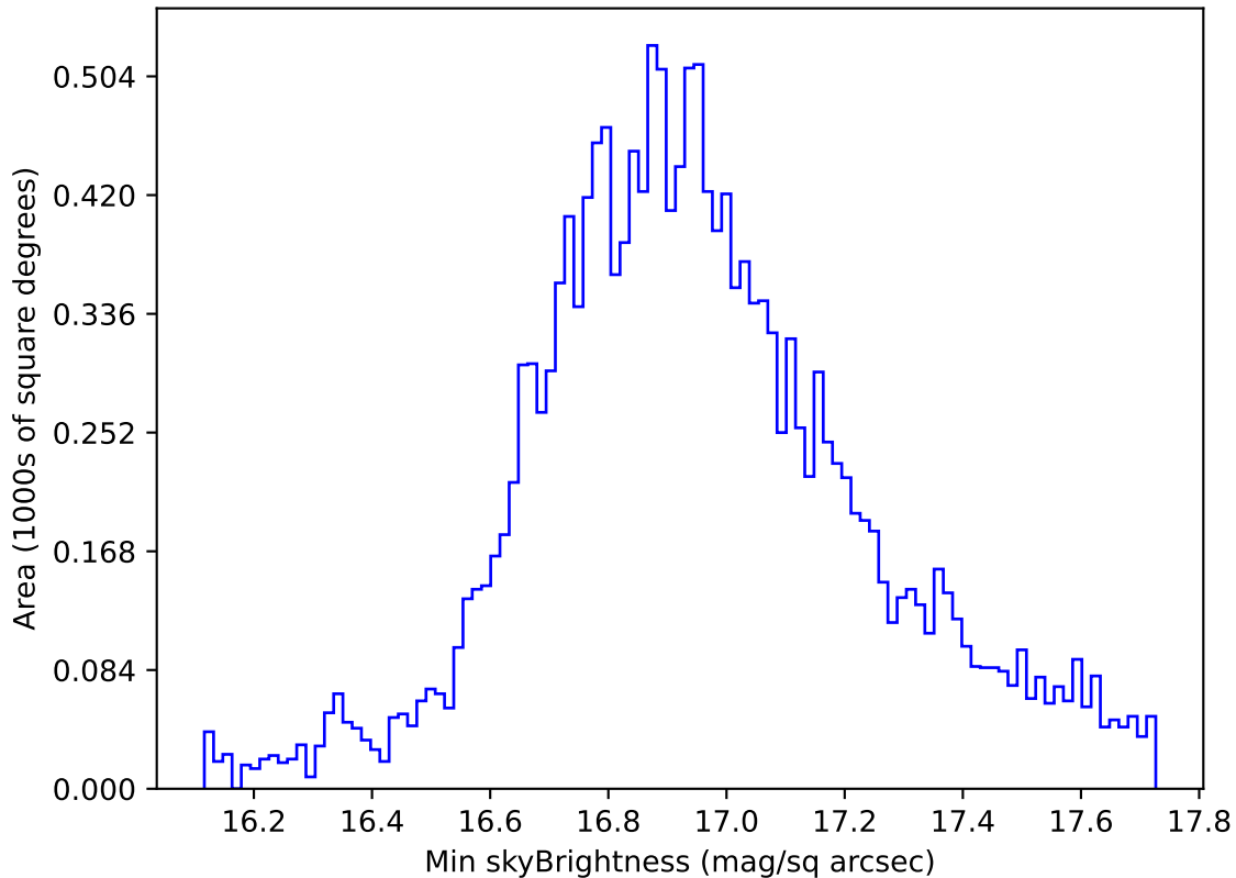
too_elab_r8_d3_giz_v3.4_10yrs WFD all bands: Min skyBrightness
