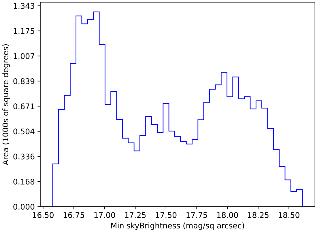
too_elab_r8_d3_giz_v3.4_10yrs All sky z band: Min skyBrightness
